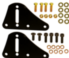
ENGINE MOUNT ADAPTER PLATES 4008 55-72 LS1 99.95 Pair
